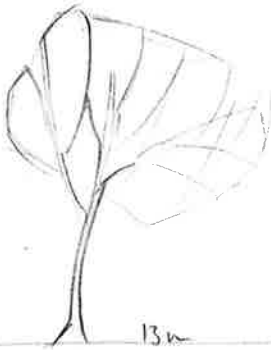
BLACK POPLAR
