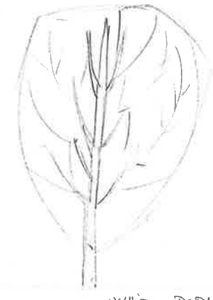
WHITE POPLAR
